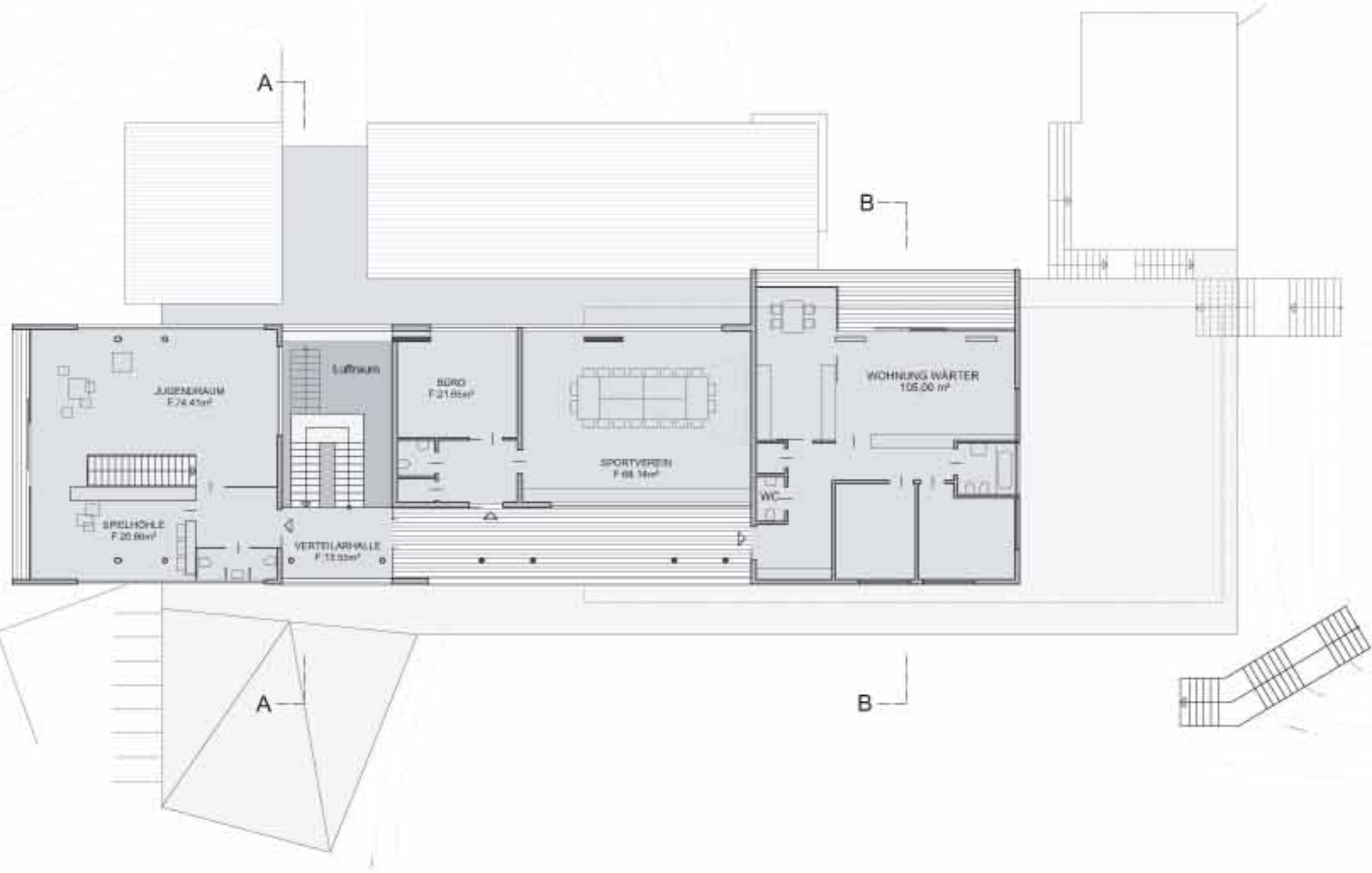
GRUNDRISS EBENE +1
